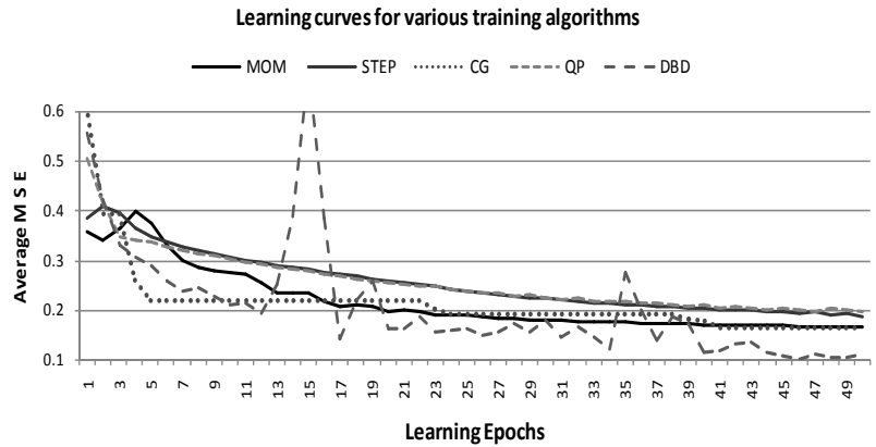
Fig. 6. Comparison of classification accuracy and MSE based on different training algorithms
