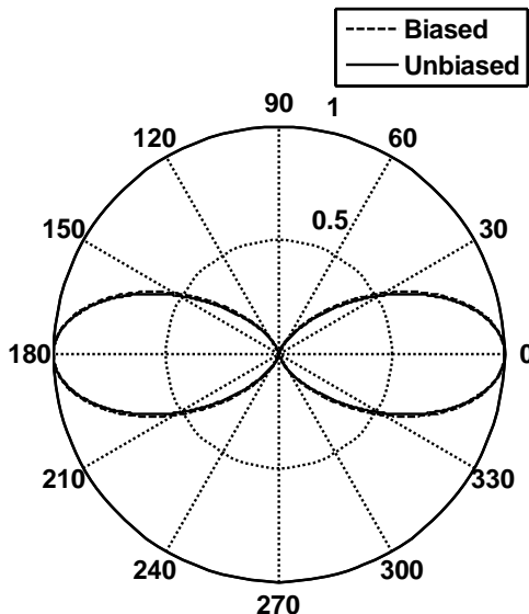
Fig. 4. Comparison of H-plane pattern of circular patch microstrip antenna with RHCP for biased case & unbiased case
