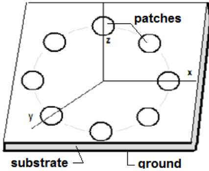
Fig. 1. Geometry of eight elements circular array microstrip circular patch antenna
