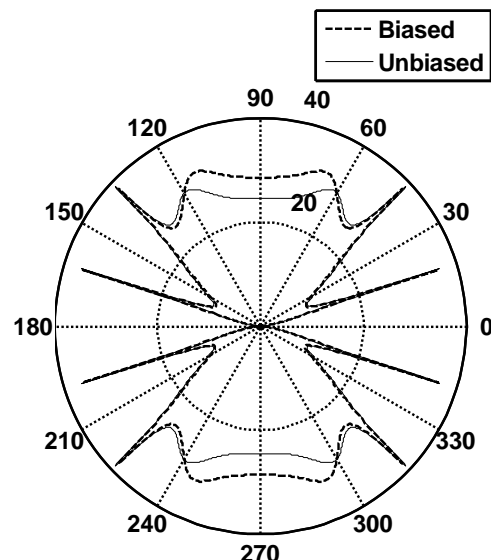
Fig. 5. Comparison of radiation pattern of 8 elements circular array of circular patches microstrip antenna with RHCP for biased and unbiased case
