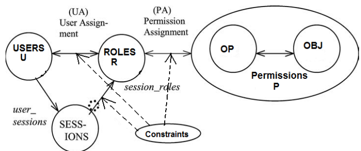
Fig. 1. RBAC System
