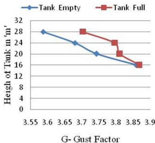
Fig. 3. Variation of gust factor for water towers of different heights
