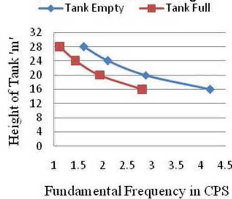
Fig. 2. Resonant component (SE/β) For water towers of different heights
