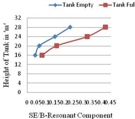
Fig. 3. Variation of gust factor for water towers of different heights
