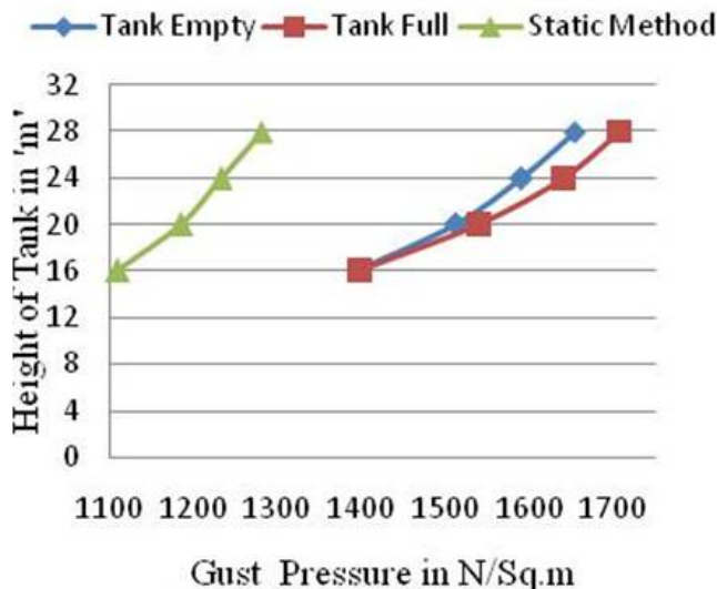
Fig. 4. Variation of gust pressures For water towers of different heights
