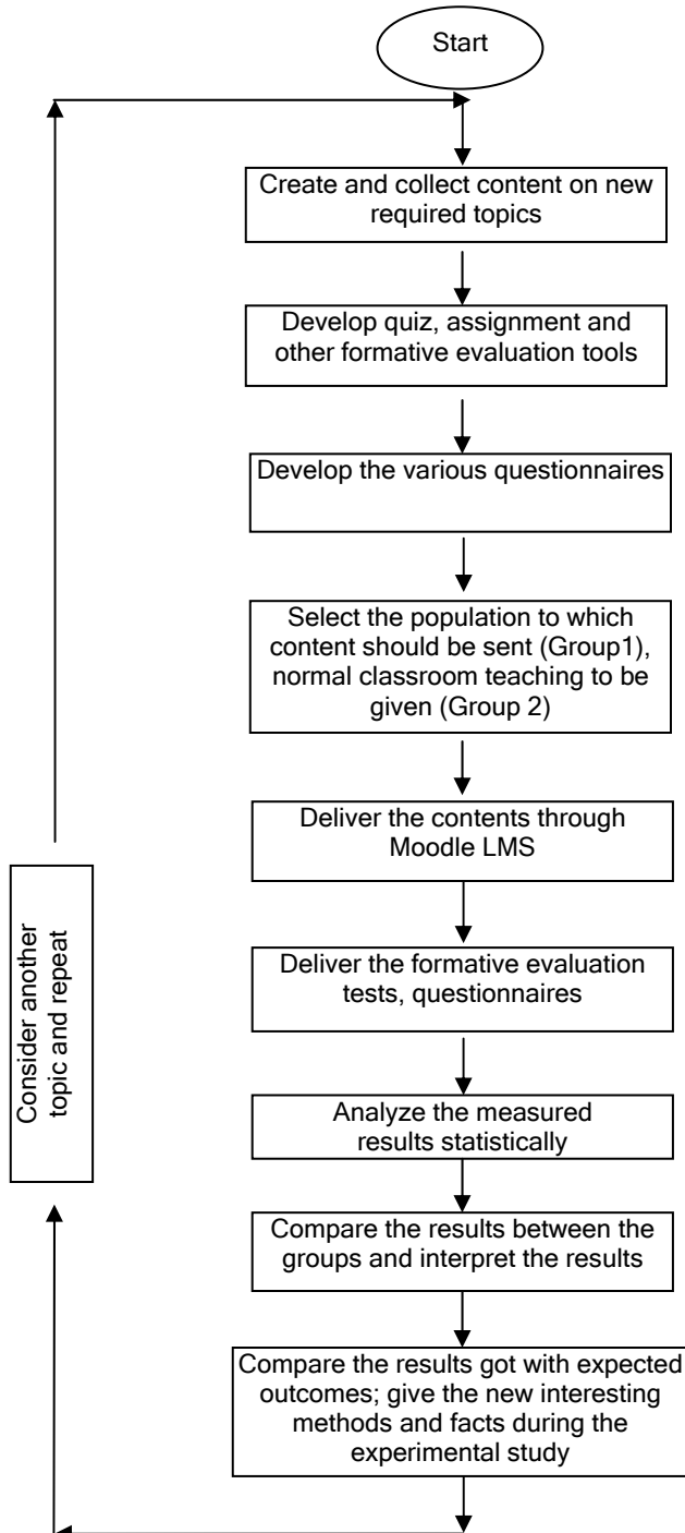
Fig. 1. Flowchart & methodology.
