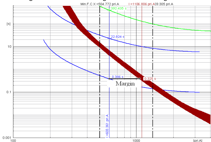
Fig. 4. Coordination margin after connecting DG
