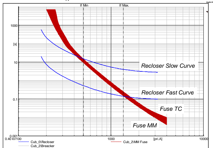
Fig.2. Recloser-Fuse coordination
