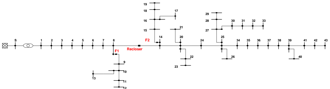
Fig. 5. Single line diagram of the studied distribution feeder in DlgSILENT Power Factory 13.2
