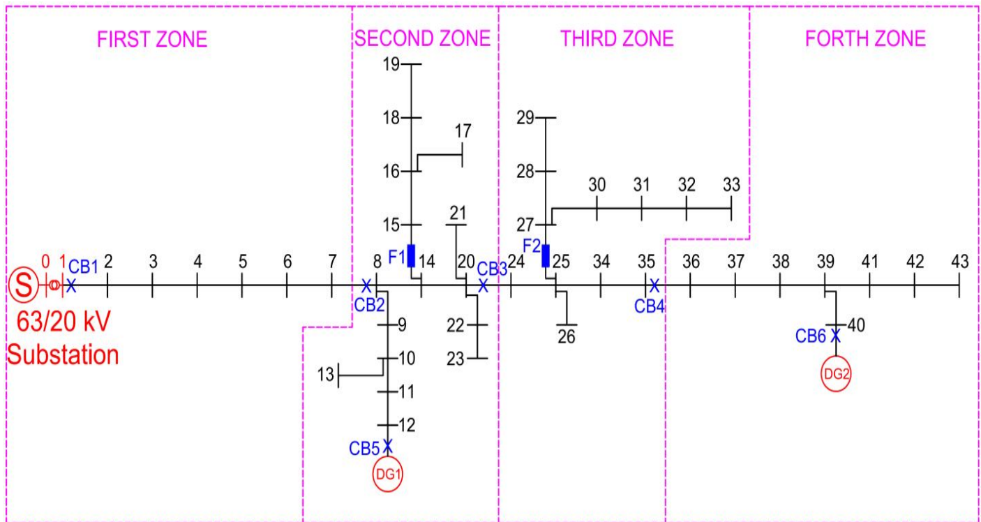
Fig.7. Single line diagram of the studied distribution feeder and its zoning after connection of DGs in the second scenario
