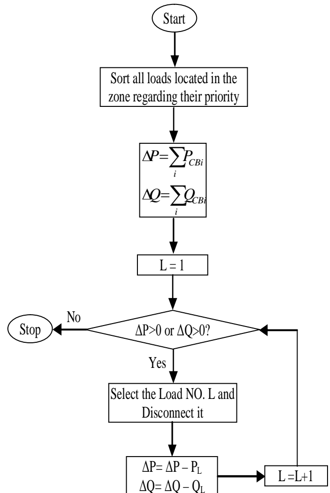
Fig.3. Load shedding algorithm of the main relay
