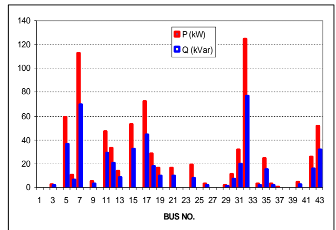
Fig.6. Load of feeder's buses in its average load regime
