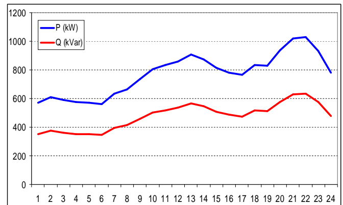
Fig.6. Load of feeder's buses in its average load regime
