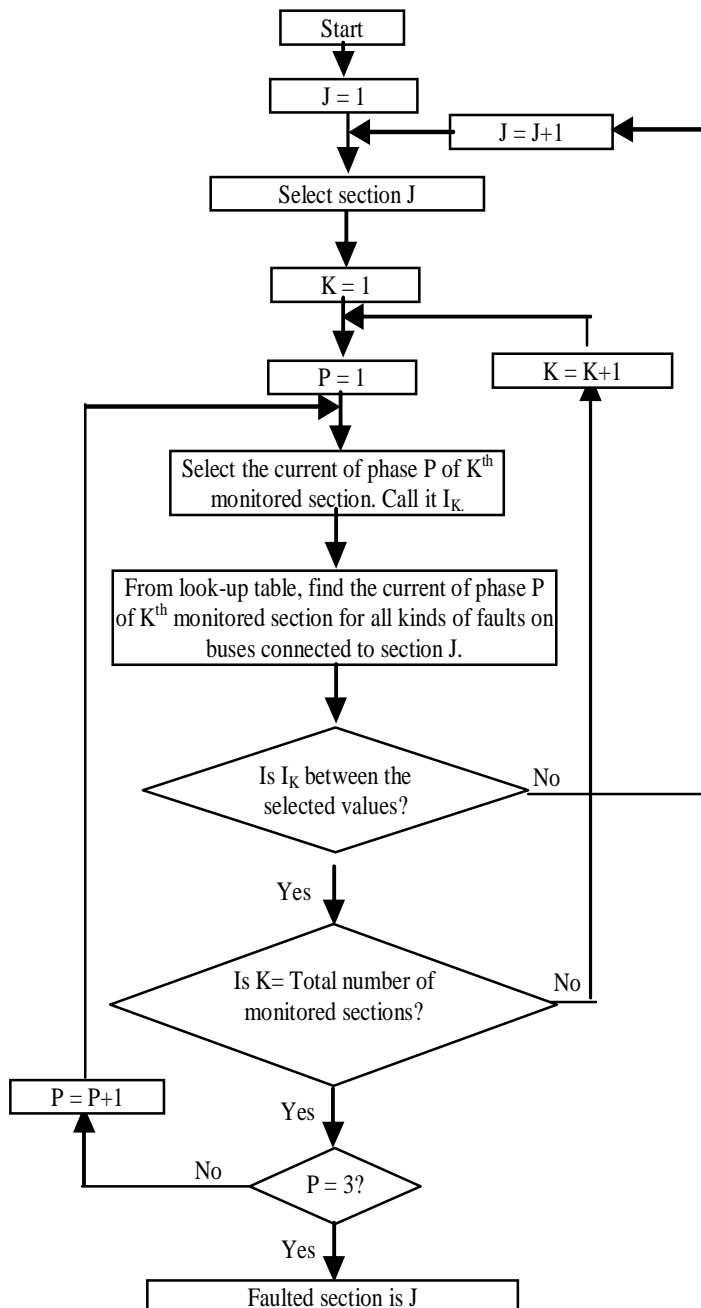
Fig.2. The algorithm for determination of fault location
