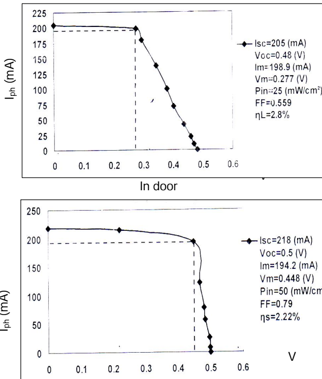
Fig.7. Comparison between output parameters for bear solar cell at indoor and outdoor measurements
