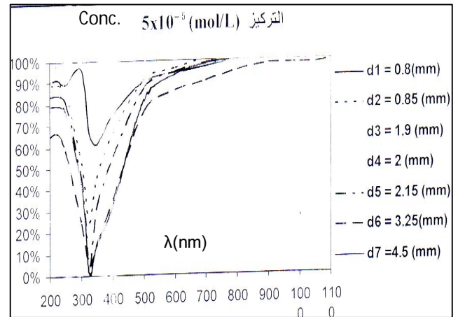
Fig.9. Relation of transmittance and wavelength for (LSC) plates in concentration ( 5 \times 10^{-5} mol/L) and in different thickness (d)
