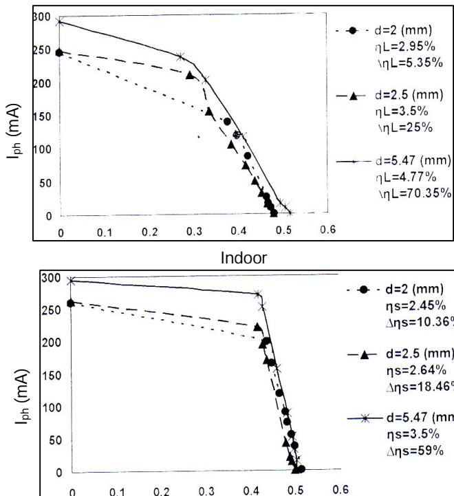
Fig.8. Comparison between conversion power efficiency by use pure epoxy plates and bare solar cell at indoor and outdoor measurements
