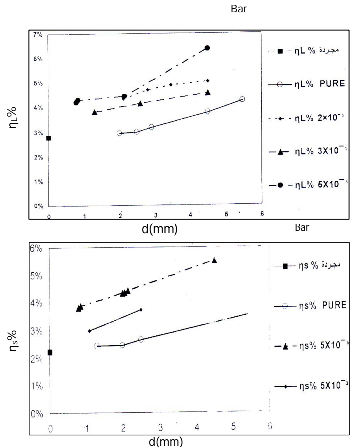
Fig.10. Increasing in conversion power efficiency with increasing (LSC) plates thickness of different concentration at indoor and outdoor measurements
