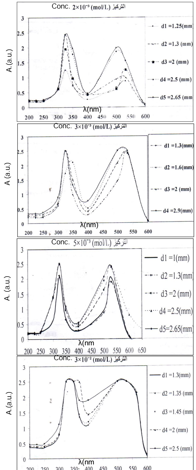
Fig.6. Relation between absorption and wavelength of (LSC) plates in different thickness ( d ) and concentration
