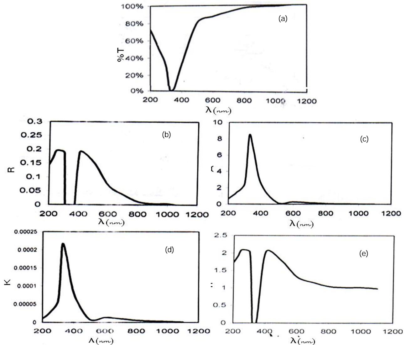
Fig.4. Optical properties and optical constant of pure epoxy plate at thickness (d) = 4.5(mm)
