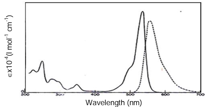
Fig.2. Absorbance and fluorescence spectrum of R6G
