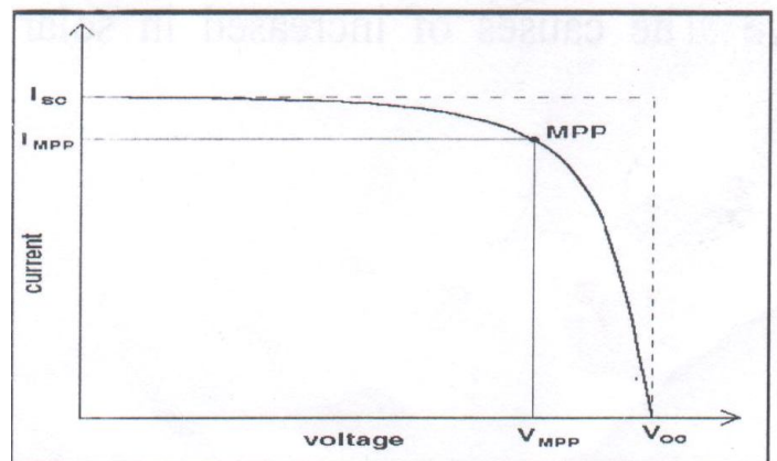
Fig. 1. Maximum power of the solar cell (MPP)
