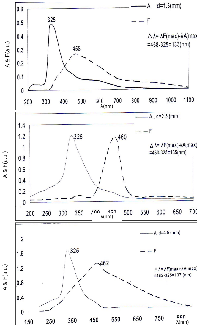
Fig.5. Stoke shift ( \Delta\lambda ) between top absorption spectrum and top fluorescence spectrum for pure epoxy plate in different thickness ( d )
