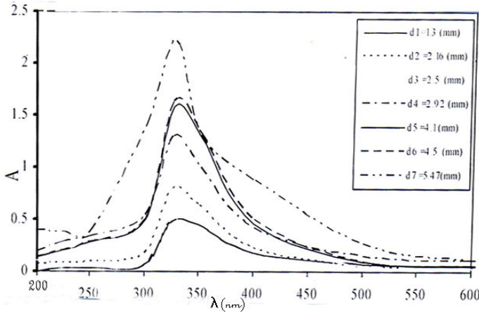
Fig.3. Absorption spectrums of pure epoxy plates in different thicknesses (d), \lambda_{(max)}=325(nm)
