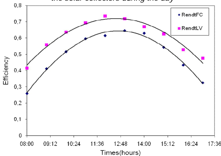
Fig. 7. Evolution of the thermal return on the solar collectors during the day
