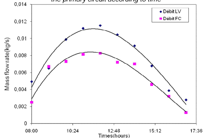
Fig.8. Evolution of the water mass flow rate in the primary circuit according to time
