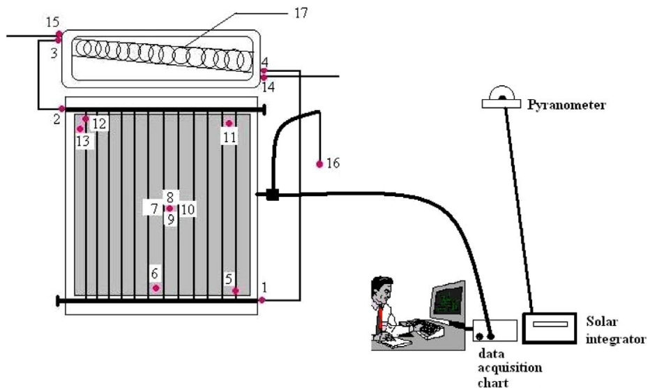
Fig. 2. Various points of measure of the temperatures and the protocol of acquisition of data
