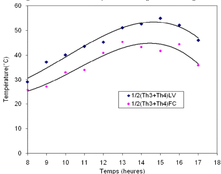
Fig. 5. Evolution of the temperature averages in the storage
