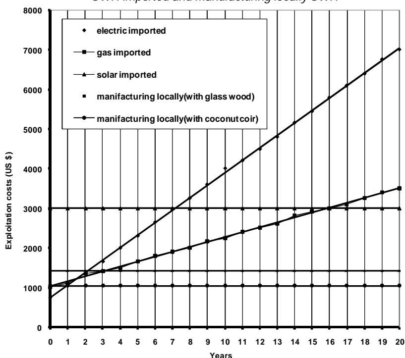
Fig.9. Comparative life cycle costs for electric, gas, SWH imported and manufacturing locally SWH
