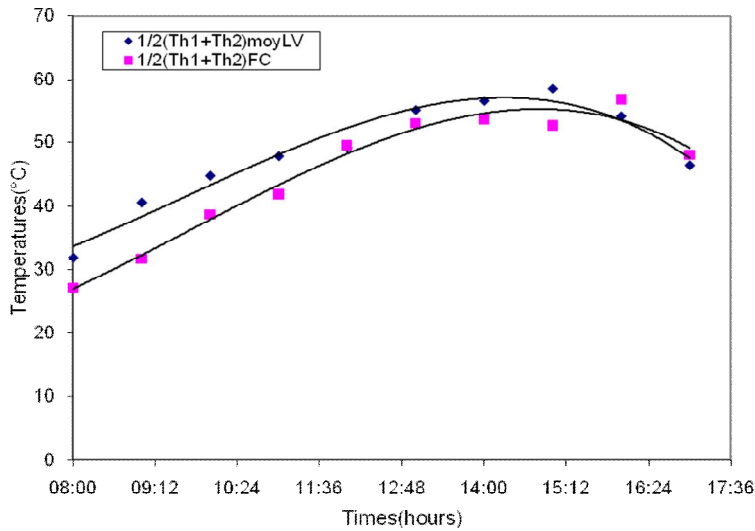
Fig. 5. Evolution of the temperature averages in the storage
