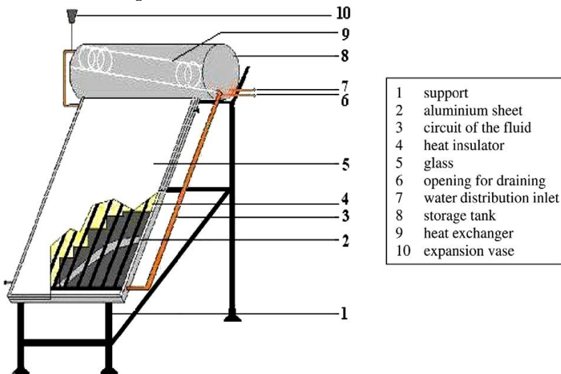
Fig. 1. Model of the realized solar water heater
