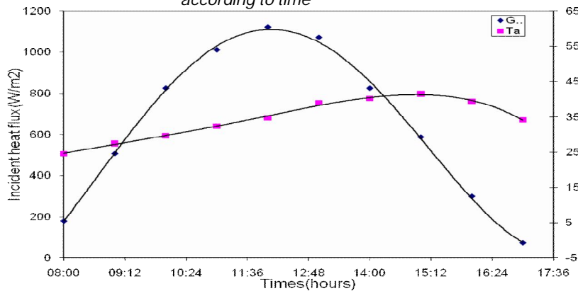
Fig.4. Evolution of the average temperatures of the solar collector
